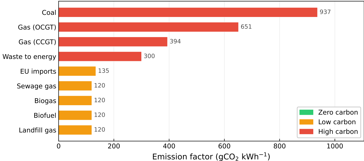
Emission Factor by Carrier
